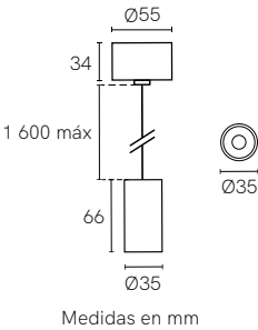
TL-9403.SUS
